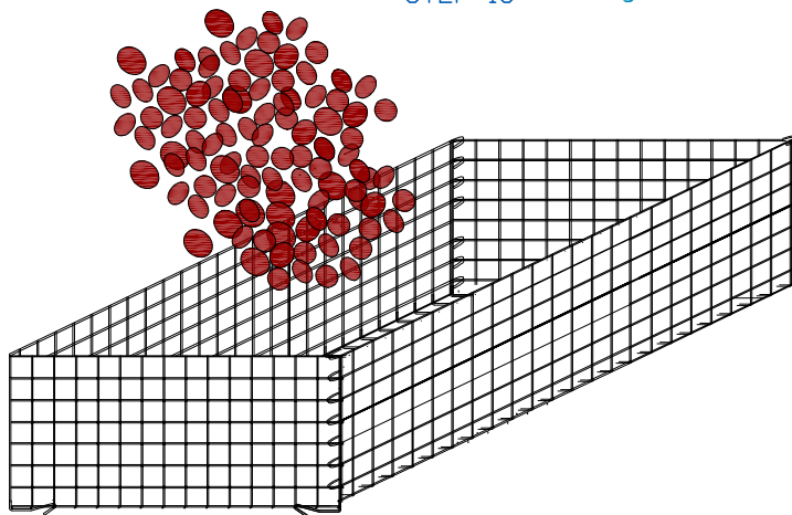
STEP 13 Filling
