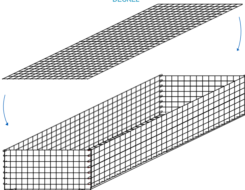
DECKEL
